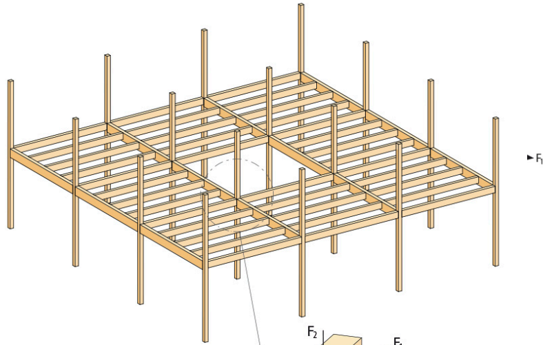
Ceiling of a timber frame construction
