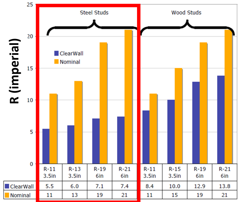
Figure 3: Nominal and Clear Wall Insulation R-values (after ASHRAE 90.1-1999) for Several Different Stud Materials and Insulation
