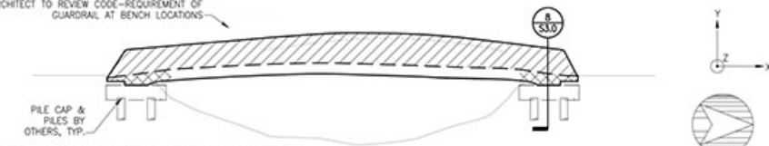
MONOLITHIC WOOD BRIDGE ELEVATION
