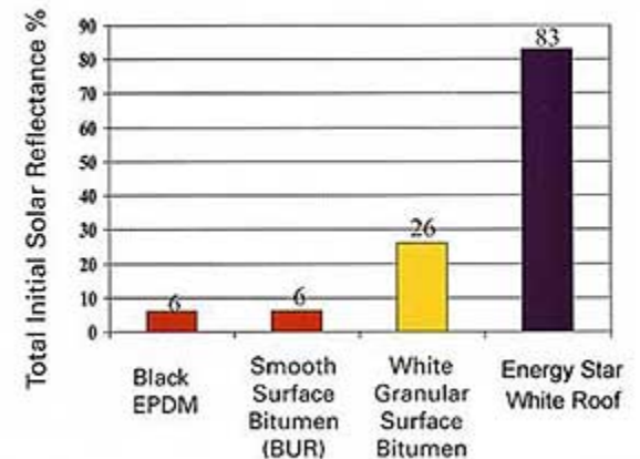
REFLECTANCE OF COMMON ROOFING MATERIALS
