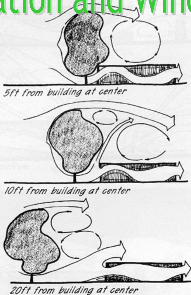
Figure 4.17: Effect on ventilation of a 30-ft tree on the windward side at different distances. (After White, 1953.)
