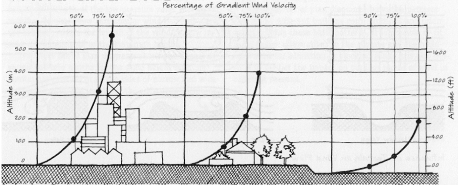
Effect of Terrain on Wind Velocity Profiles
