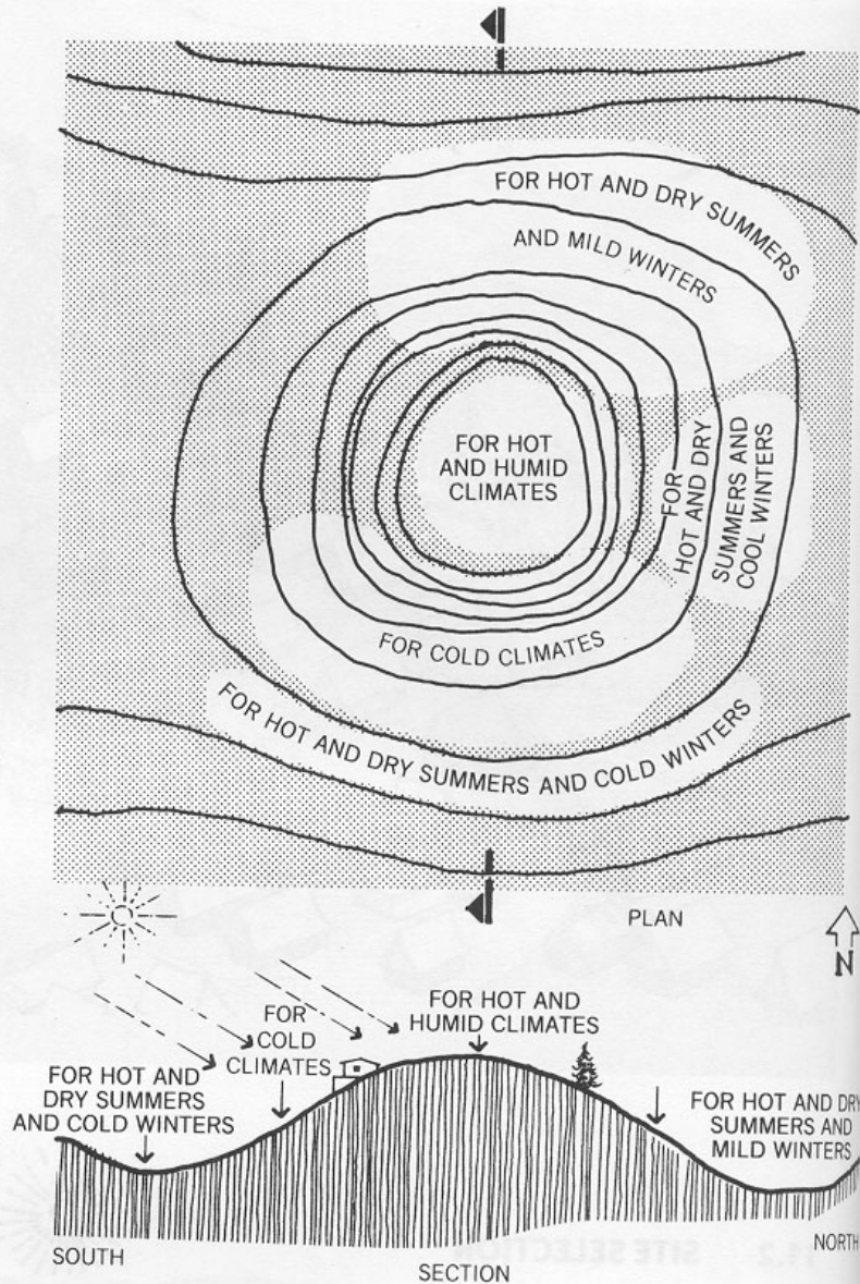
Figure 11.2d Preferred building sites around a hill in response to climate for envelope-dominated buildings.
