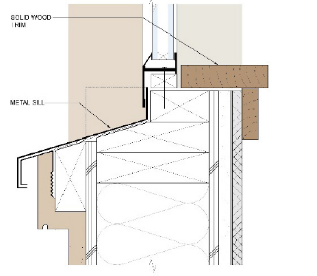
REMOVABLE WINDOW : DETAIL B
