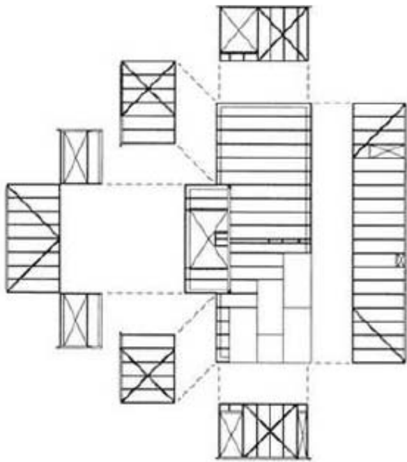
1 framing
